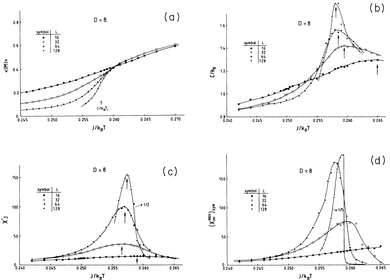
FIG. 11. Order parameter \langle |M| \rangle (a), specific heat C/k_B (b), suseptibility \chi'J (c), and maximum value of the layer susceptibility \chi_{nn}^{\max}J (d) plotted vs inverse temperature for D=8 . Several sizes of L are included as indicated.
