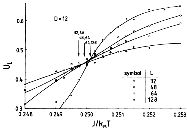
FIG. 8. Cumulants U_L [Eq. (13)] plotted vs inverse temperature for D=12 , |H_1|/J=0.55 , and several choices of L . The arrows indicate the locations of cumulant crossings of pairs of sizes. Note that J/k_B T_w \approx 0.250 for |H_1|/J=0.55 and that the bulk Ising transition at J/k_B T_{cb} \approx 0.227 is far off scale. Curves are only guides to the eye.
